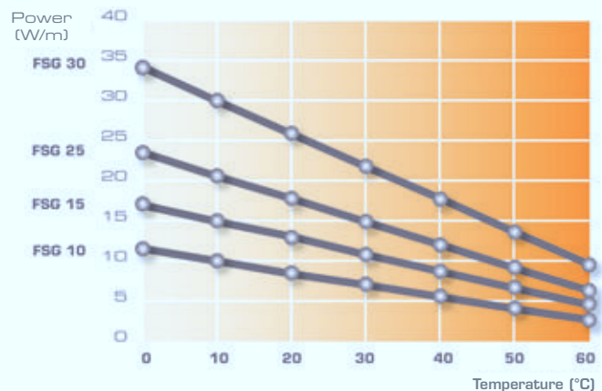
Power output according to pipe temperature
